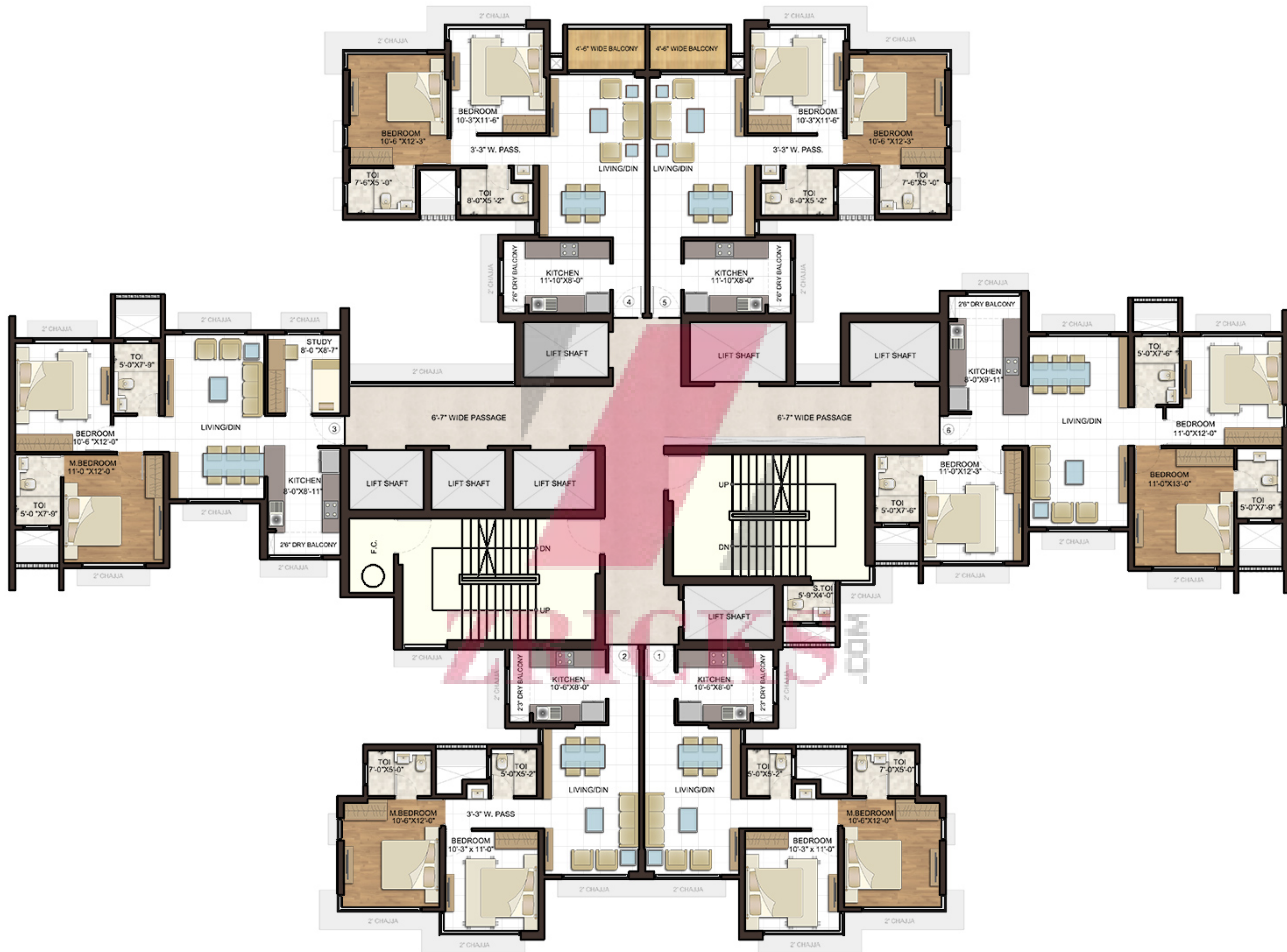
WING A: TYPICAL FLOOR PLAN (31st to 35th & 37th)
