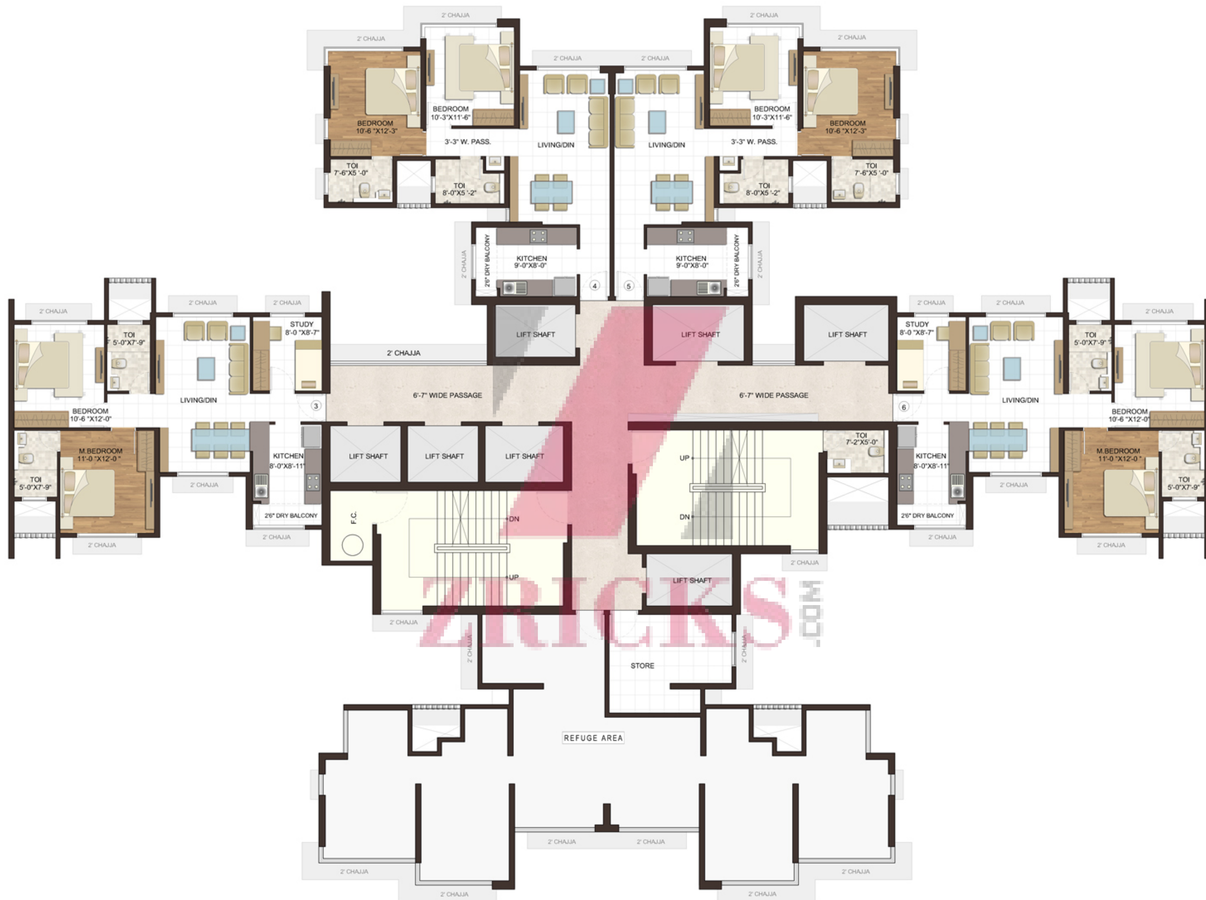
WING B: REFUGE FLOOR PLAN (8TH, 15TH, 22ND & 29TH)
