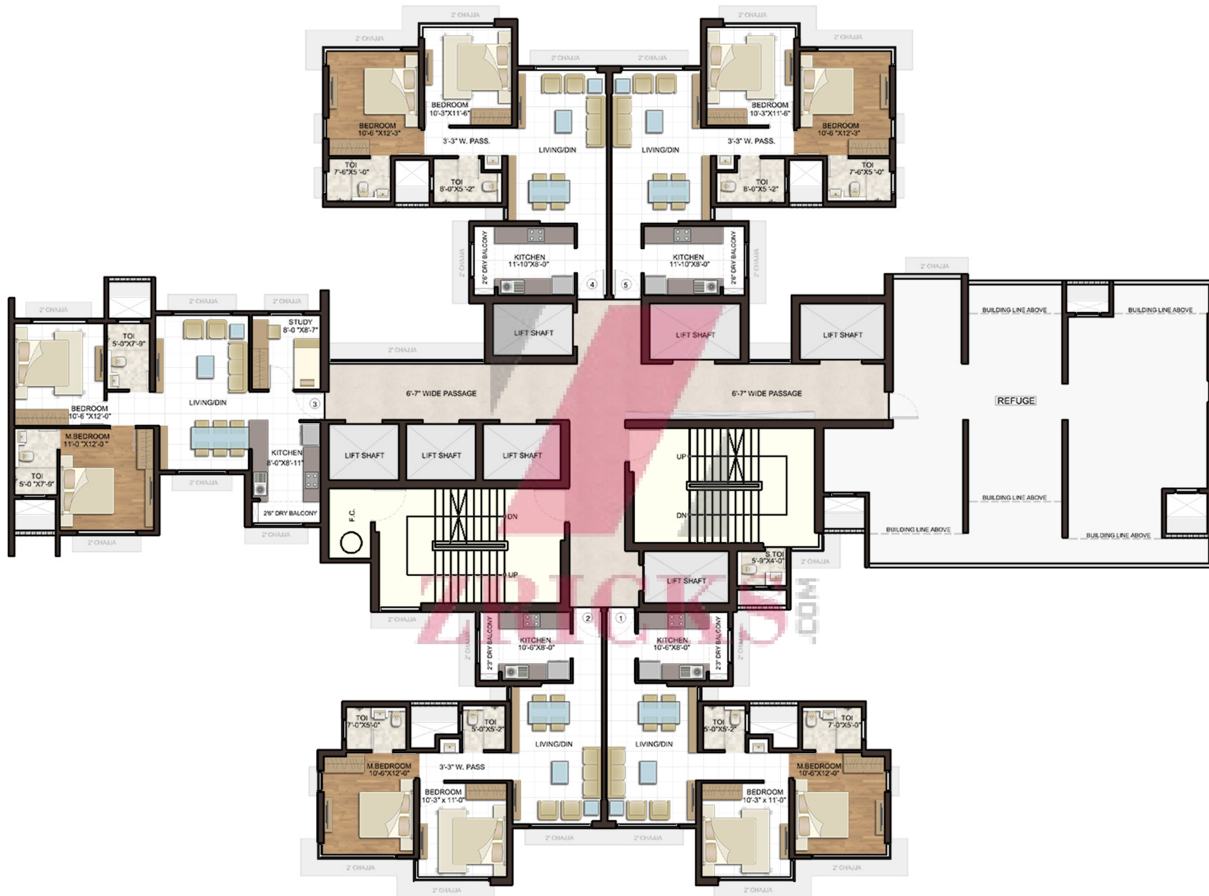
WING A: REFUGE FLOOR PLAN (8TH, 15TH, 22ND & 29TH)
